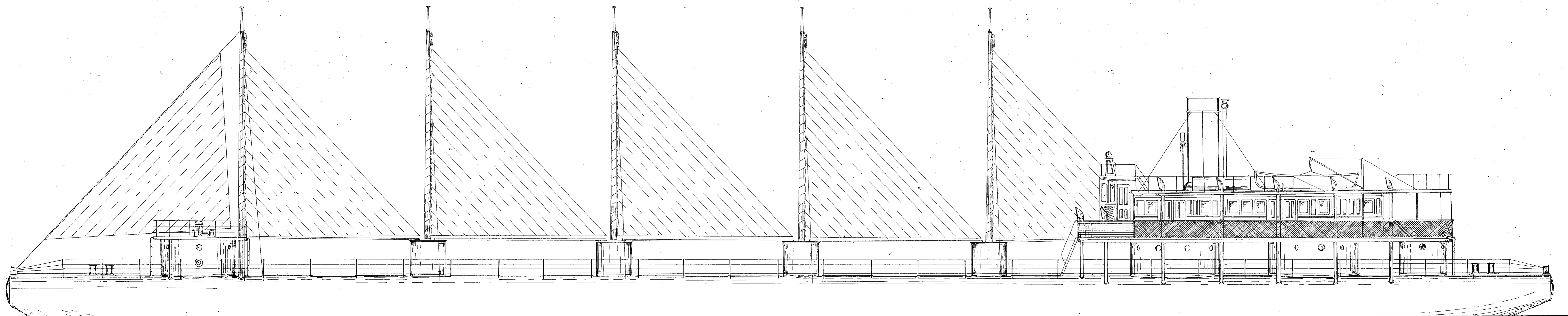
—Sail Plan of C. W. Wetmore—
